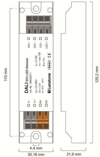
Geometrie 10A and 16A
